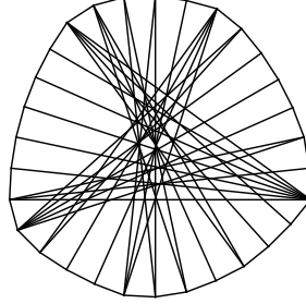
FIGURE 6. Sporadic optimal polygons for n = 30 .
