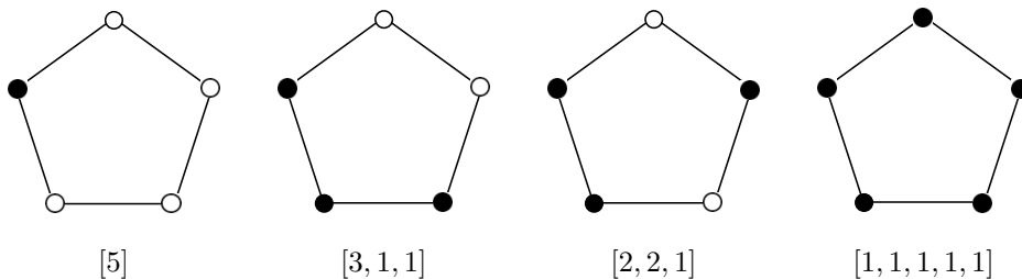
FIGURE 5. Correspondence between dihedral compositions and necklaces.
