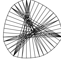
FIGURE 7. Sporadic optimal polygons for n = 42 .
