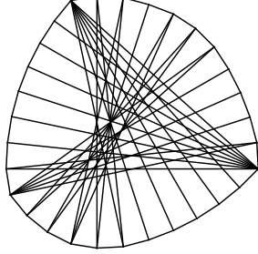
FIGURE 6. Sporadic optimal polygons for n = 30 .
