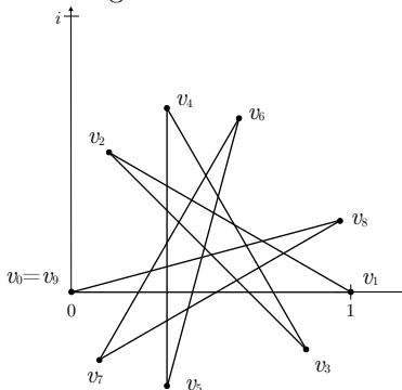
FIGURE 4. Labeling vertices on a Reuleaux polygon.
