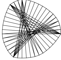
FIGURE 7. Sporadic optimal polygons for n = 42 .
