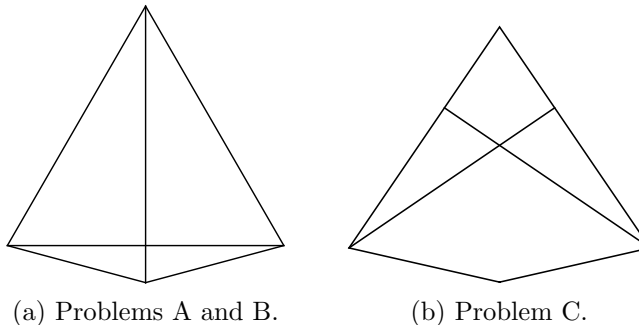
FIGURE 9. Optimal quadrilaterals.
