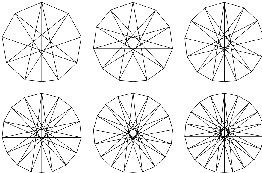
FIGURE 3. Improved polygons Q_n for n = 10 through n = 20 .
