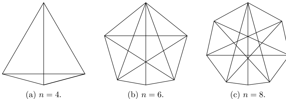
FIGURE 1. Some optimal polygons.
